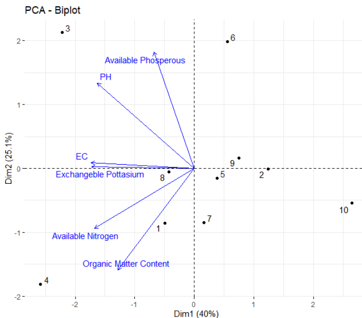
Figure 2: Principle component analysis (PCA) bi plot EC – Electrical conductivity
