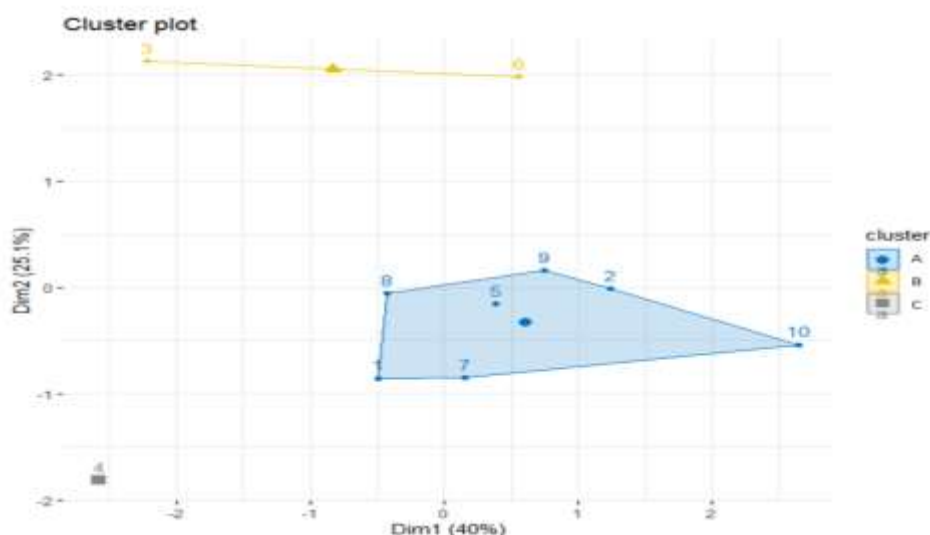
Figure 3: Cluster plot of soil samples according to collected locations 1- Siyambalanduwa, 2- Ampara, 3- Jaffna, 4- Dabana, 5- Thanamalwila, 6- Sooriyawewa, 7 Angunakolawewa, 8- Weheragala, 9- Ethimale, 10- WUSL
