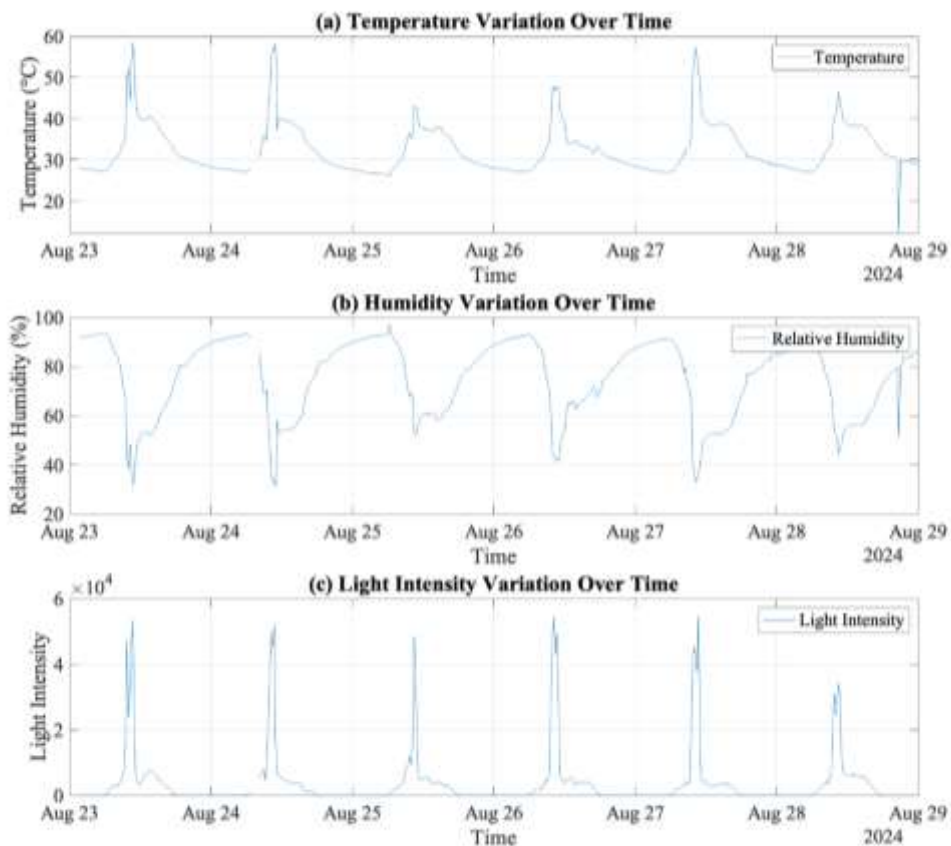
Figure 3: Weather parameter variations obtained from the datalogger: a. Temperature, b. Humidity, c. Light Intensity, variations over time.
