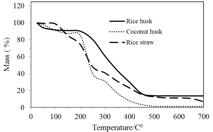
Figure 1: TGA curves for Rice husk, Coconut husk and Rice straw
